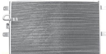
FAB-33000 Condenser Ford BA Falcon 10/02-2/08 Core: 632 / 378 / 16
