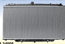
NGR-34005 Radiator PA ATM 13mm Bleed Pipe No Overflow Stub Nissan Y61 PATROL 2.8/3.0L Core: 450 / 908 / 36
